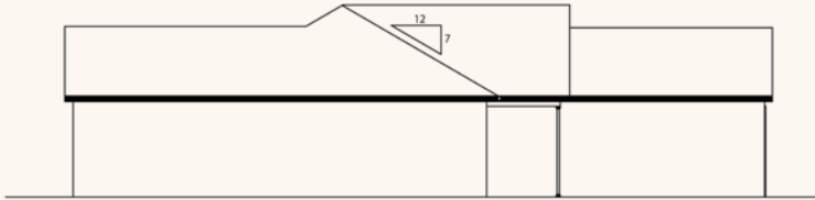
LEFT ELEVATION
